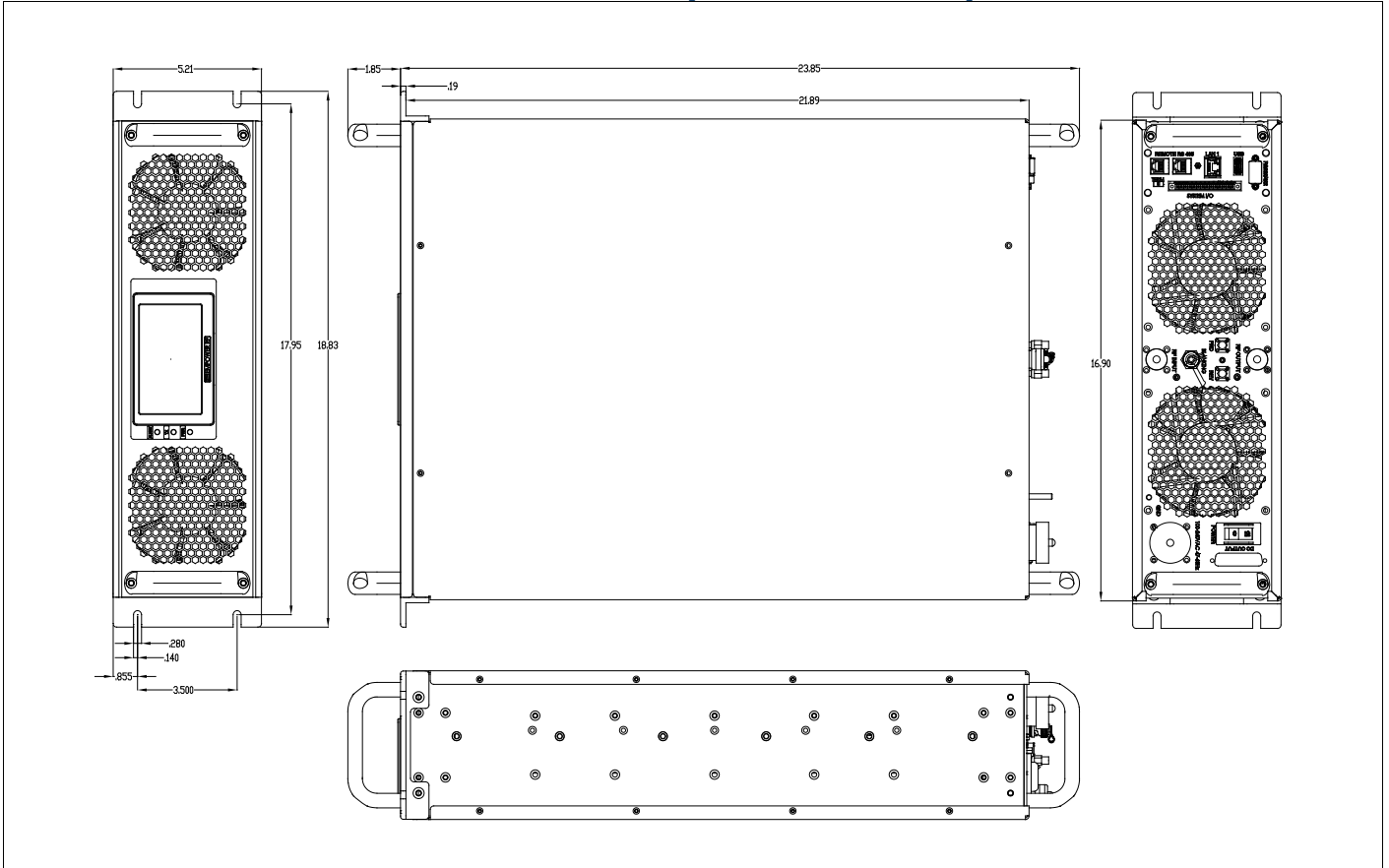
MECHANICAL OUTLINE [with rear RF connectors]
