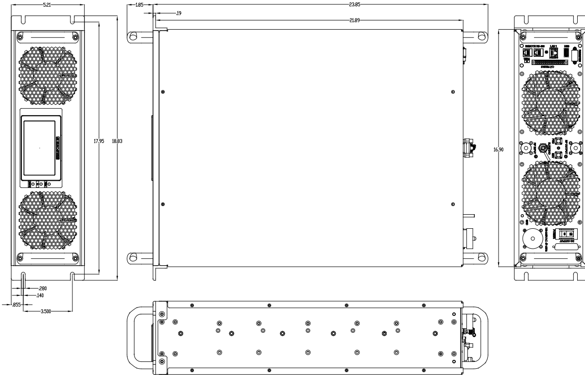
OUTLINE DRAWING (Shown with rear RF connectors)
