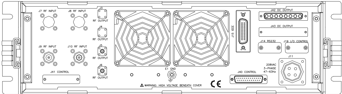
SYSTEM OUTLINE DRAWING - REAR VIEW
