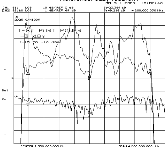
Plot 3 – Gain Adjustment Range
