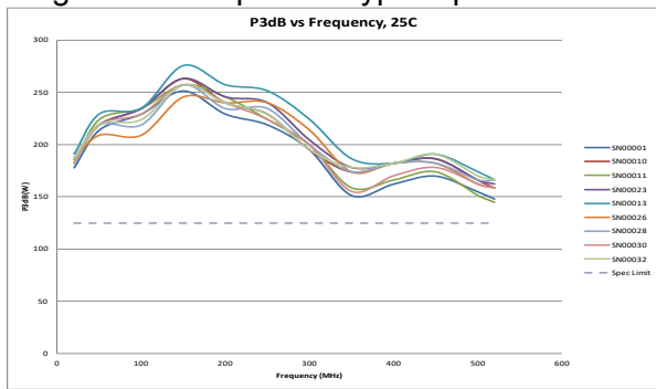
Figure 2: IS95, 9 channel forward P_{3dB} performance over frequency for 9 units. V_{SUPPLY} is 28V. Base plate temperature is 25 C.
