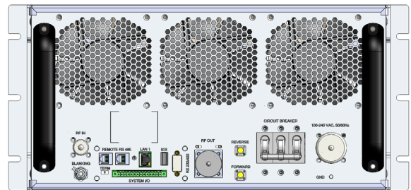
2126-008 Rear View
